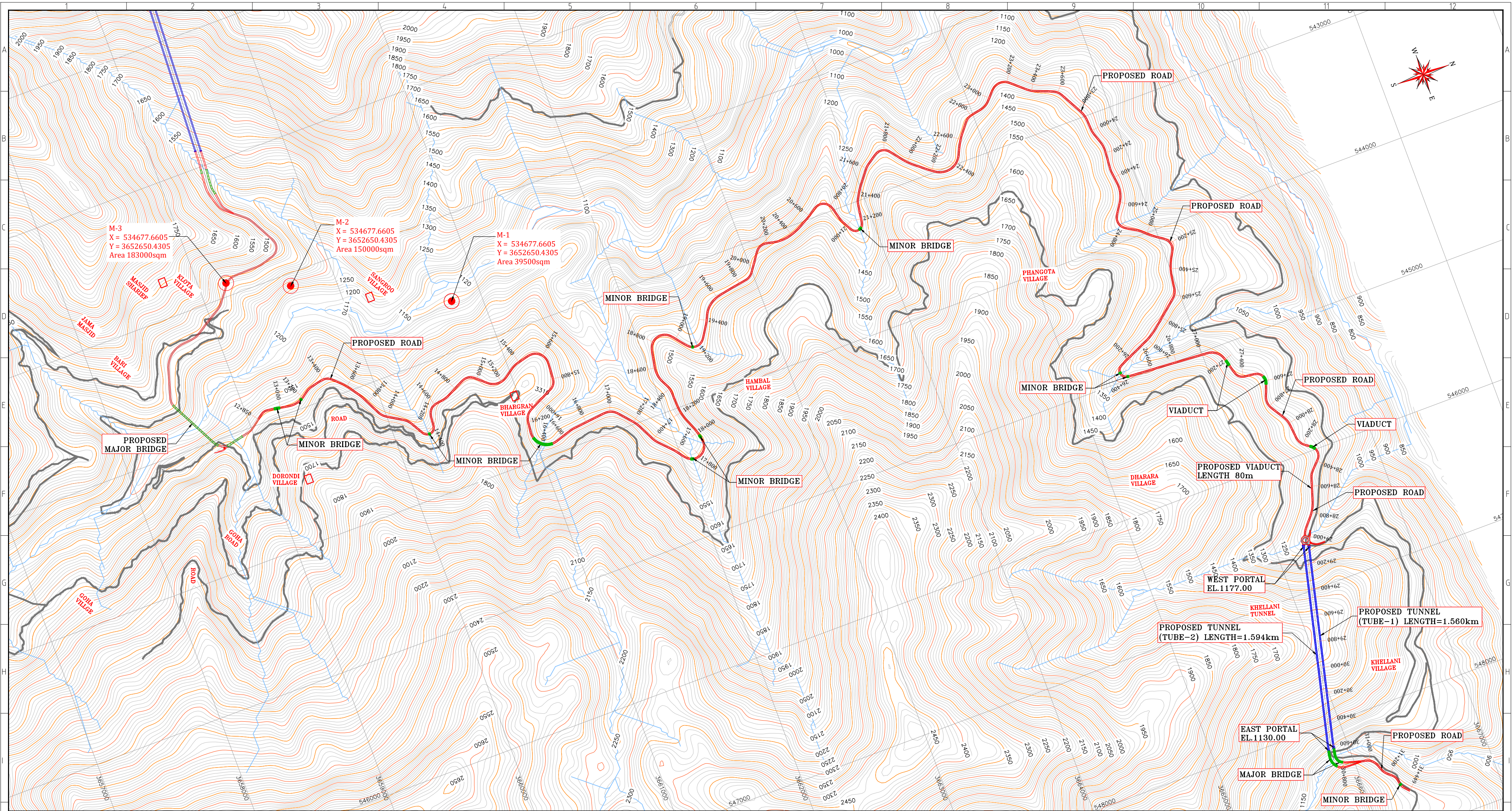
LAYOUT PLAN
